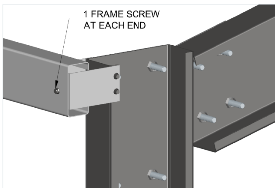
EAVE PURLIN CONNECTION AT END WALL COLUMN
