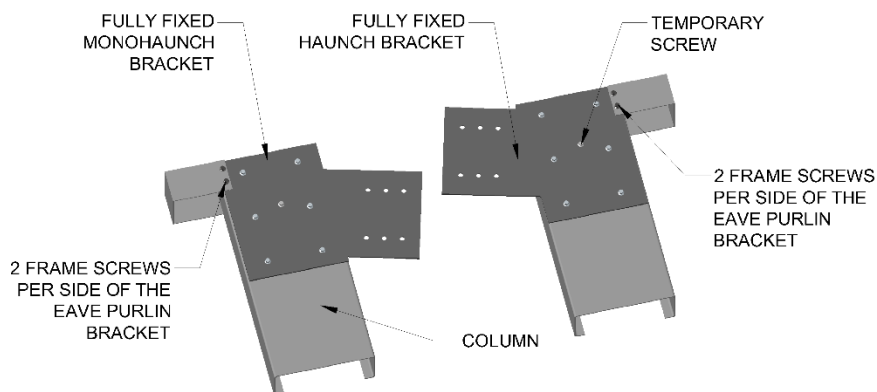
FITTING OF SINGLE COLUMNS WITH HAUNCH BRACKET
