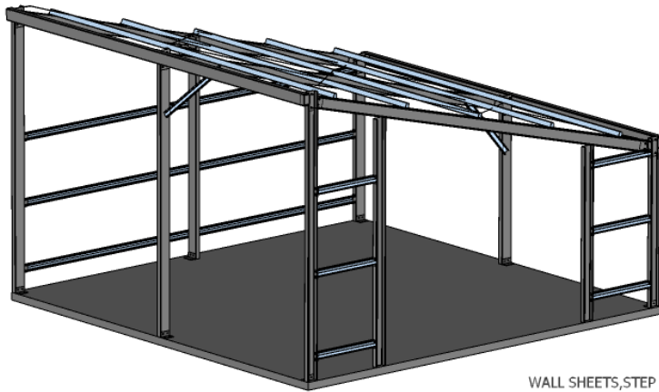
FIXING OF ENDWALL GIRTS
