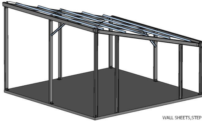
FIXING OF ROOF PURLINS
