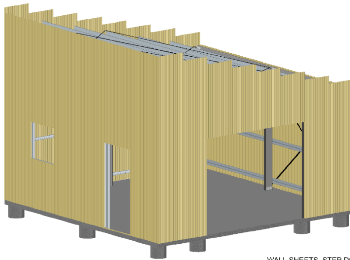
FIXING OF END WALL SHEETS
