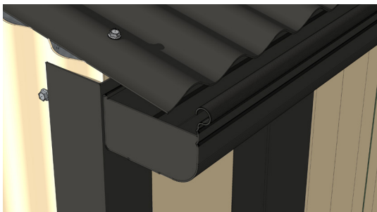
Overhang gutter by approx. 50mm
